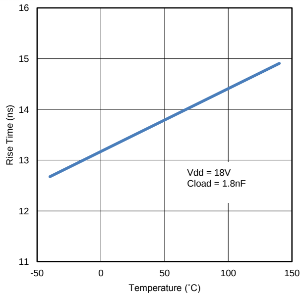
Figure 29. Rise Time vs. Temperature
