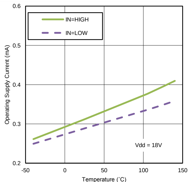
Figure 26. Operating Supply Current vs. Temperature (output in DC on/off condition)
