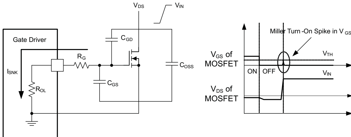
Figure 36. Low Pull-Down Impedance in UCC2753x (output stage mitigates Miller turn-on effect)
