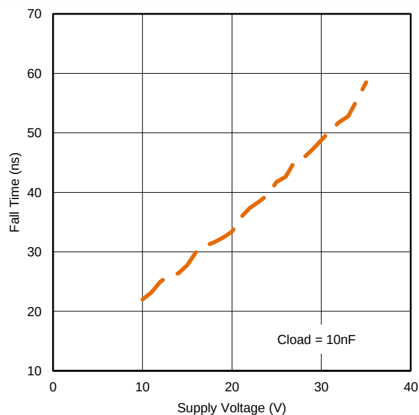
Figure 33. Fall Time vs. Supply Voltage
