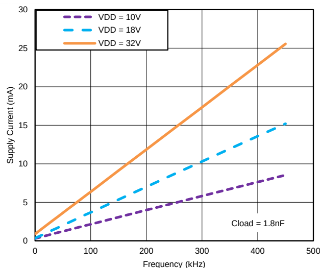
Figure 17. Operating Supply Current vs. Frequency
