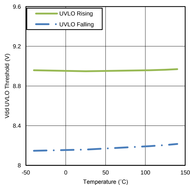
Figure 20. UVLO Threshold Voltage vs. Temperature
