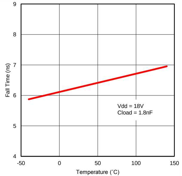
Figure 30. Fall Time vs. Temperature
