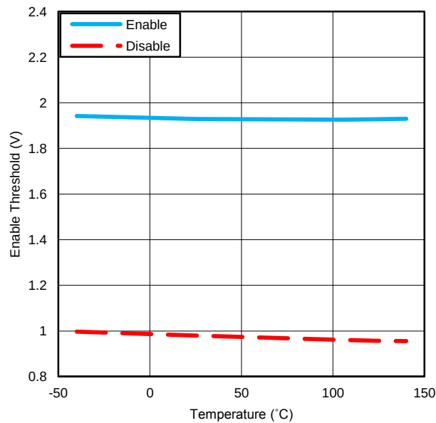
Figure 23. Enable Threshold vs. Temperature
