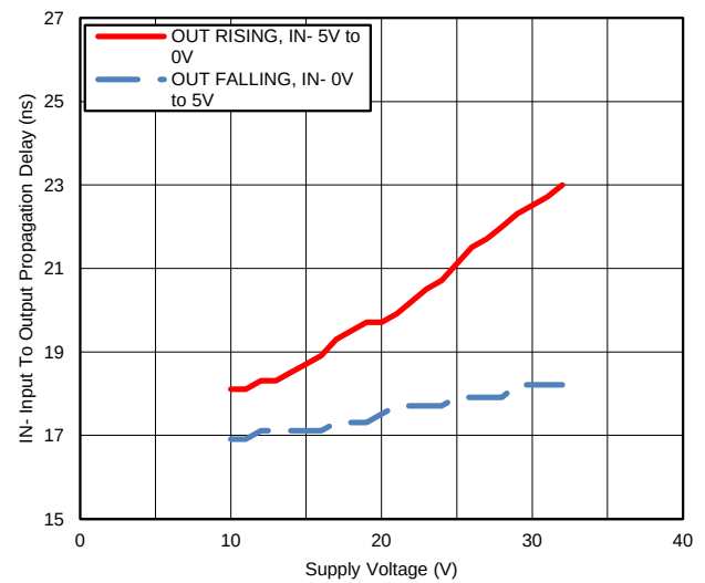
Figure 16. IN- Propagation Delay vs. Supply
