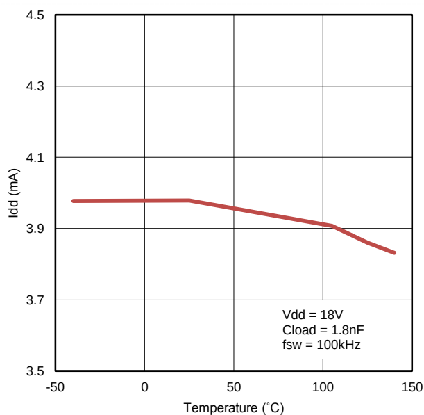
Figure 19. Operating Supply Current vs. Temperature (output switching)
