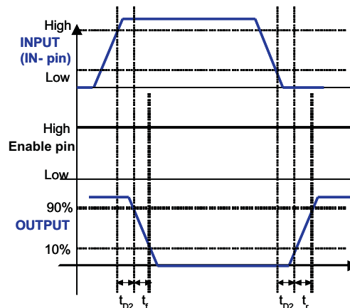
Figure 3. UCC27537: (OUTPUT = OUT) ENABLE = IN+ UCC27538: (OUTPUT = OUT) ENABLE = EN
