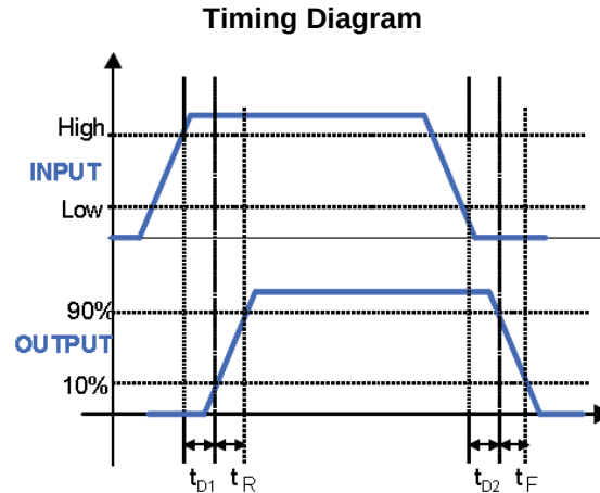
Figure 1. UCC27531: (OUTPUT = OUTH tied to OUTL) INPUT = IN, (EN = VDD), or INPUT = EN, (IN = VDD) (OUTPUT = OUT) INPUT = IN+, (EN = VDD), or INPUT = EN, (IN+ = VDD) (OUTPUT = OUTH tied to OUTL) INPUT = IN1, (IN2 = VDD), or INPUT = IN2, (IN1 = VDD)
