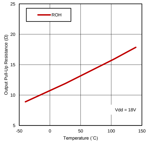
Figure 24. Output Pull-Up Resistance vs. Temperature
