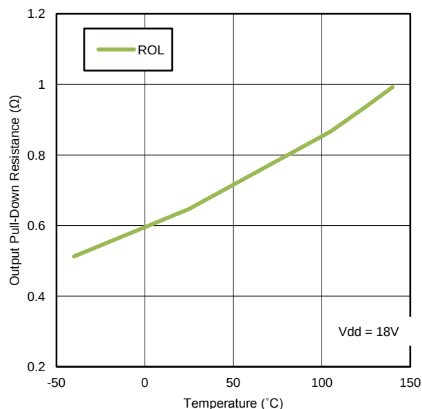
Figure 25. Output Pull-Down Resistance vs. Temperature
