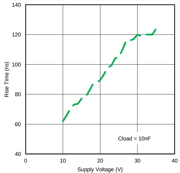
Figure 32. Rise Time vs. Supply Voltage
