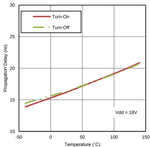
Figure 27. Input-to-Output Propagation Delay vs. Temperature
