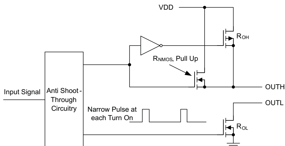
Figure 35. UCC27531 Gate Driver Output Stage
