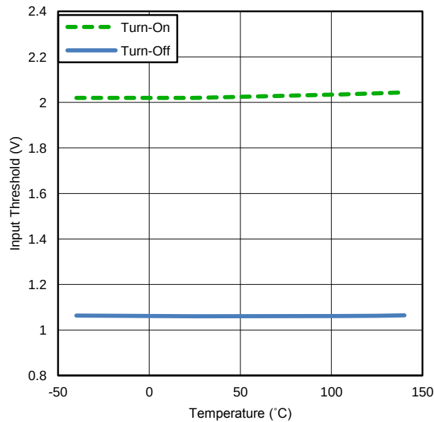
Figure 21. Input Threshold vs. Temperature
