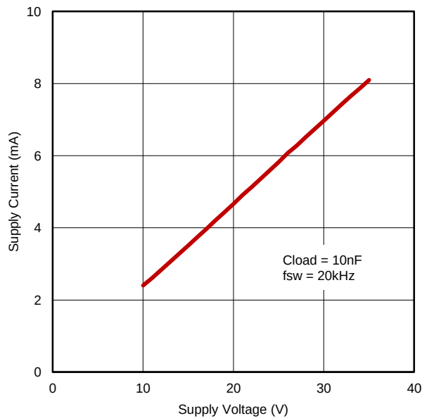
Figure 31. Operating Supply Current vs. Supply Voltage (output switching)
